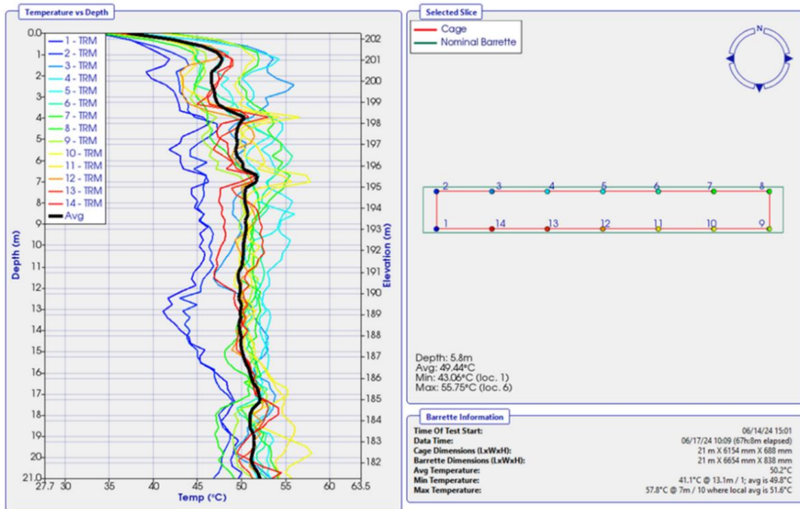
Figure 6. Thermal Integrity Profiling results for all wires in a diaphragm wall.
