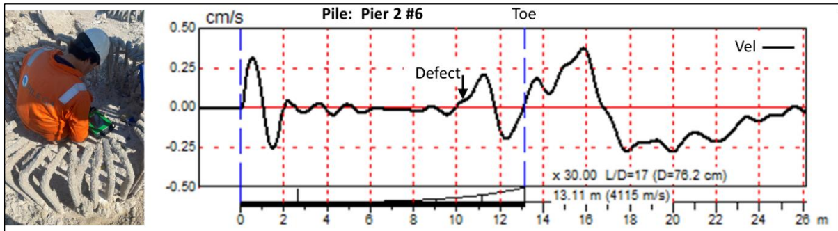
Figure 8. Photo of a PIT test (left) with an example record indicating a defect at 10.2m depth.
