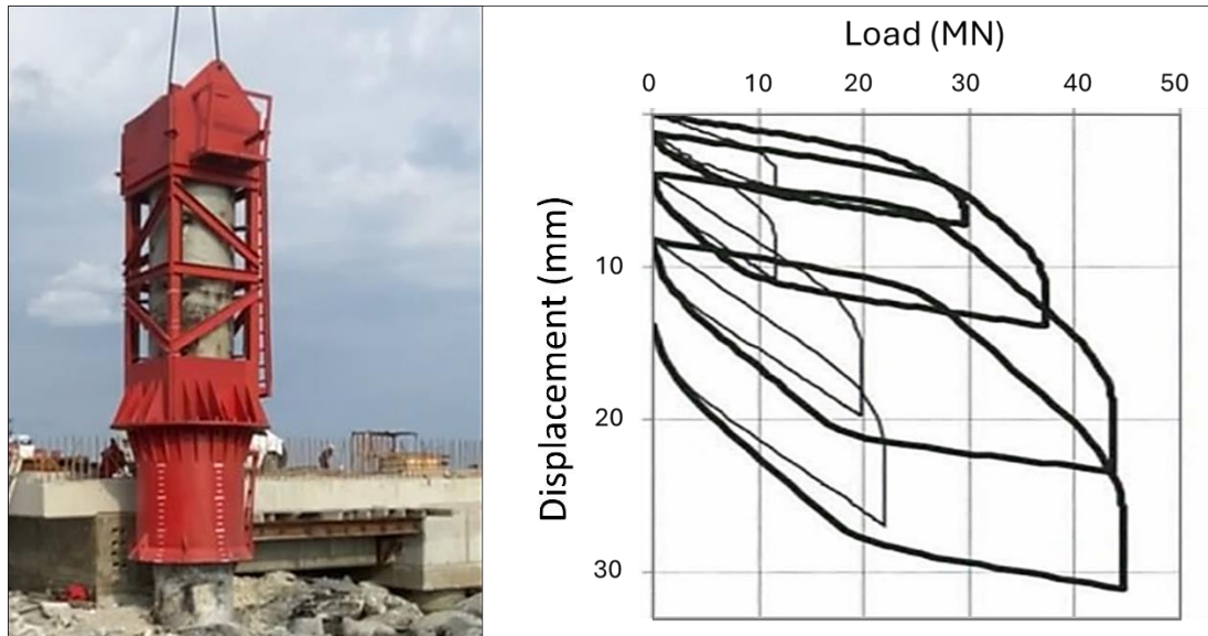
Figure 9. Dynamic load test on bored pile (left) and example test results (right).
