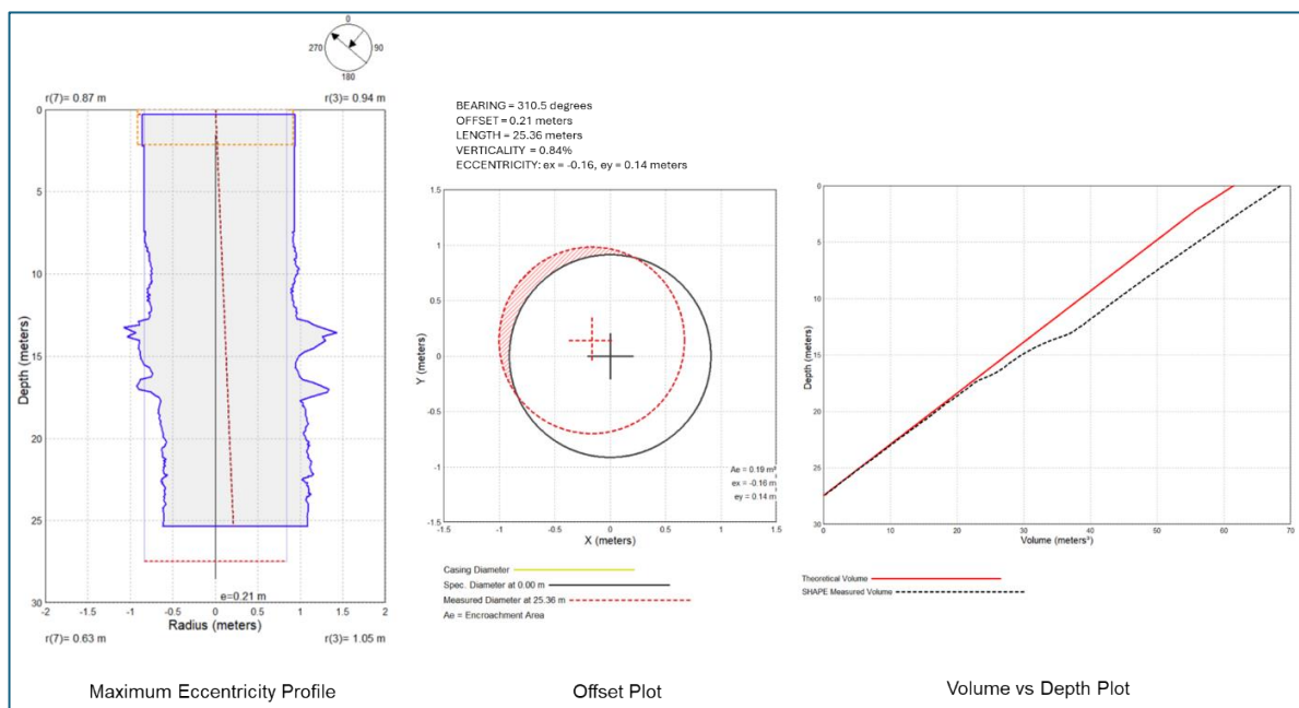
Figure 2. SHAPE profile, offset, and volume vs depth plot in shaft with sidewall instability.
