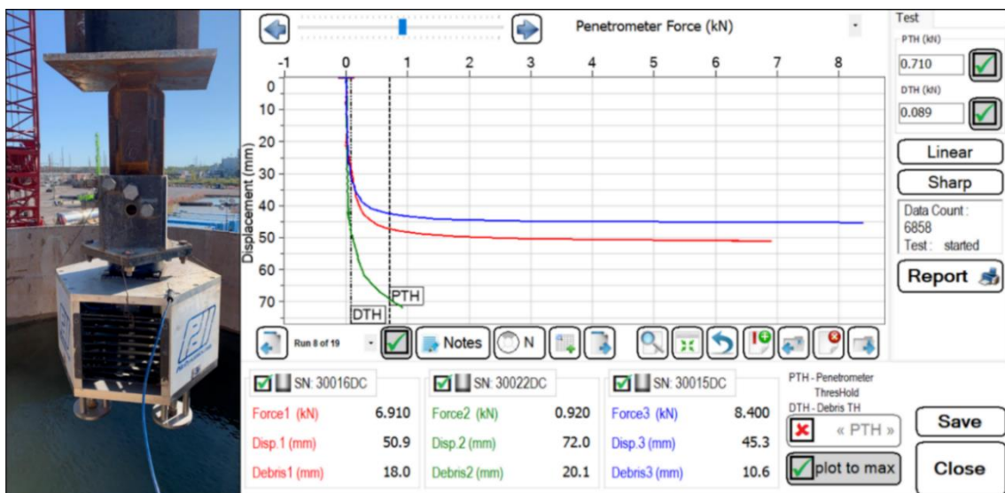
Figure 4. SQUID system attached to weighted beam on crane line (left) and test results (right).
