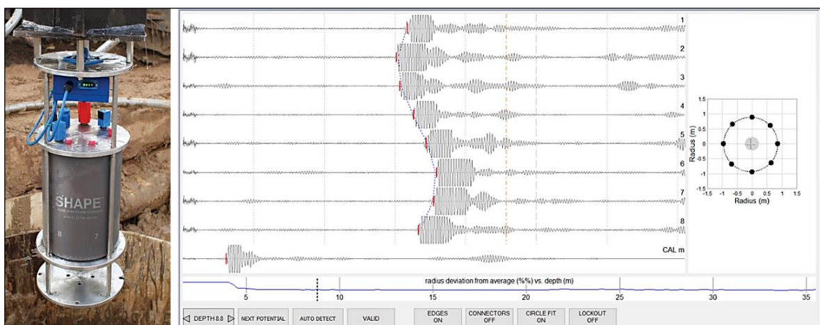
Figure 1. SHAPE device (left) and test results at one test depth from each sensor (right).
