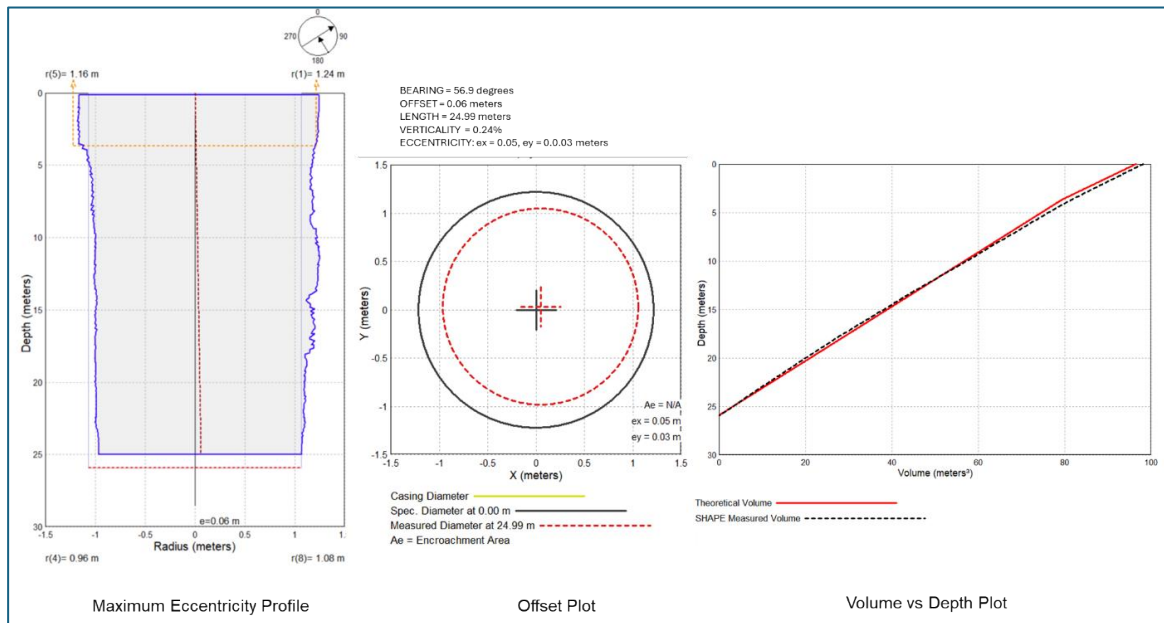
Figure 3. SHAPE profile, offset, and volume vs depth plot for well controlled installation.
