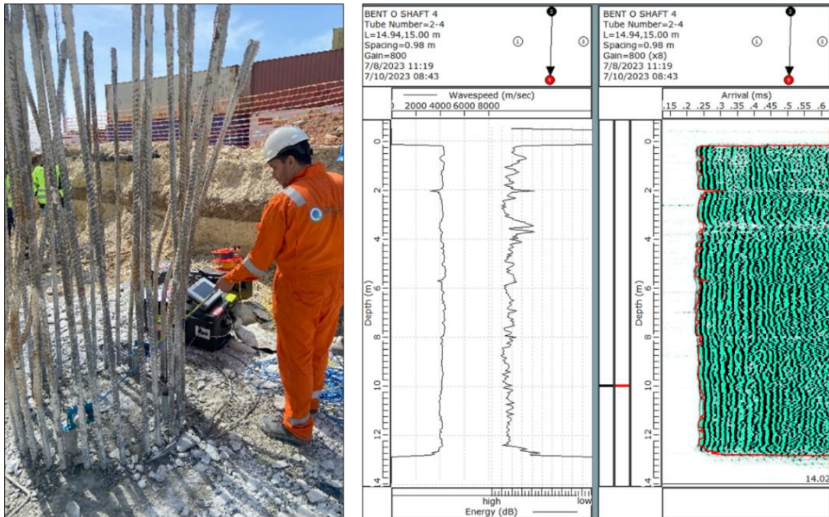
Figure 7. CSL test (left), first arrival time and energy (center) and FAT waterfall (right) vs depth plots.
