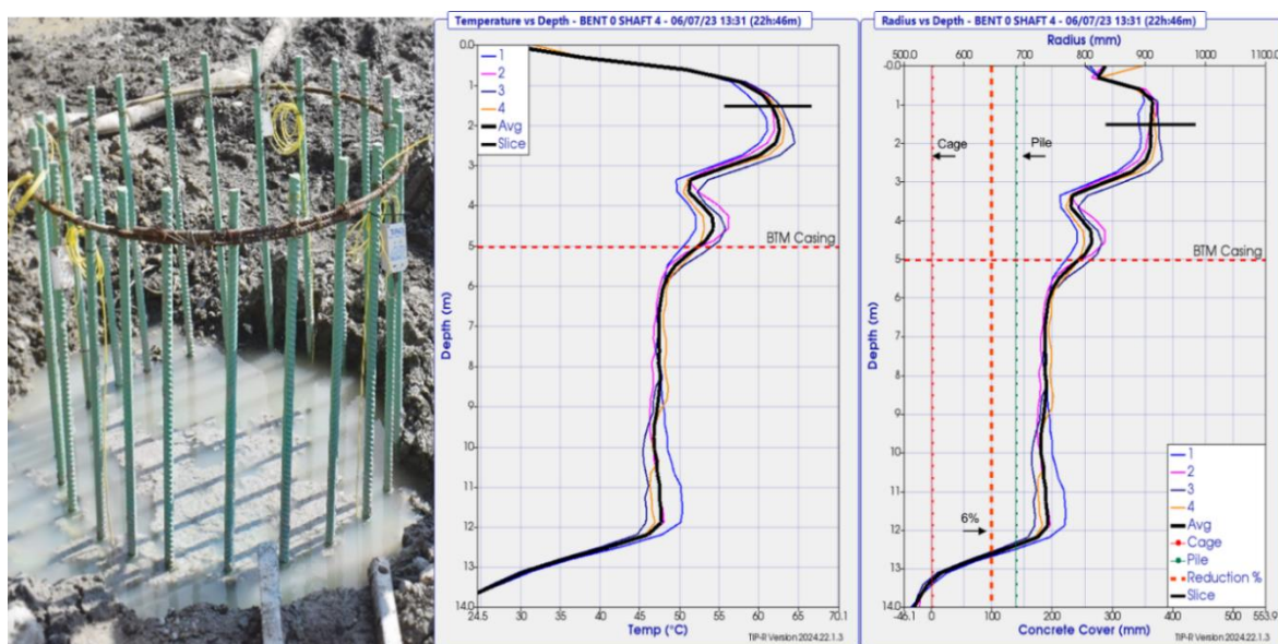
Figure 5. TIP equipment (left), temperature vs depth (center) and effective radius vs depth (right).
